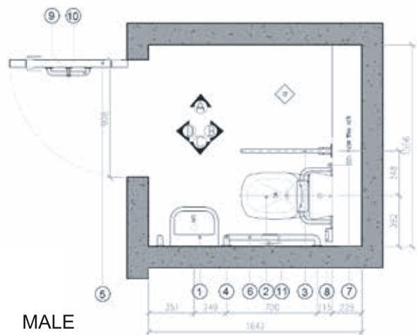
PWD TOILET FLOOR PLAN SCALE: 1:20 mm
